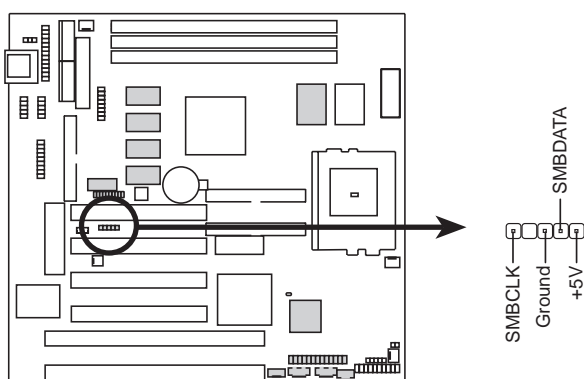
P5S-B SMBus Connector
