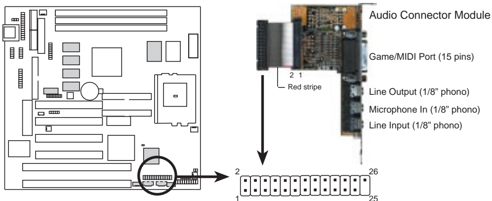
P5S-B Audio Header
