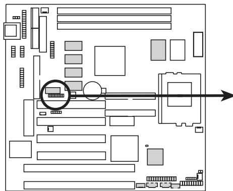
P5S-B LCD Header
