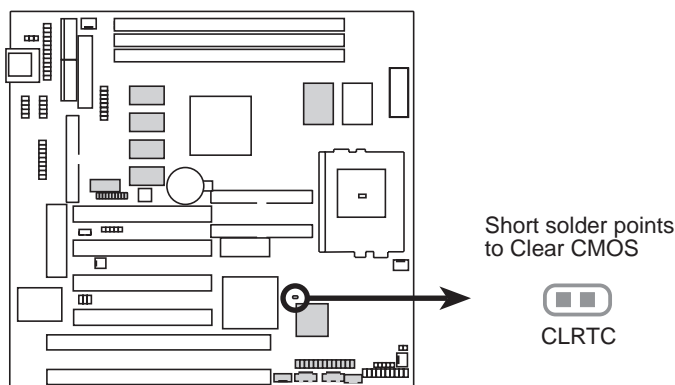
P5S-B Clear RTC RAM
