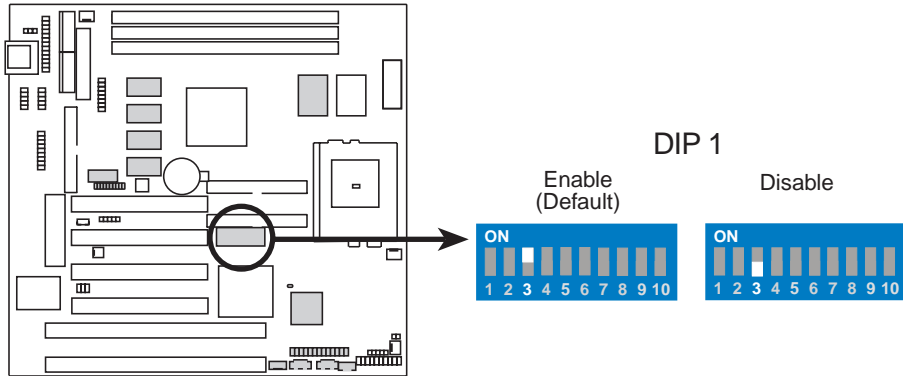
P5S-B Audio Setting
