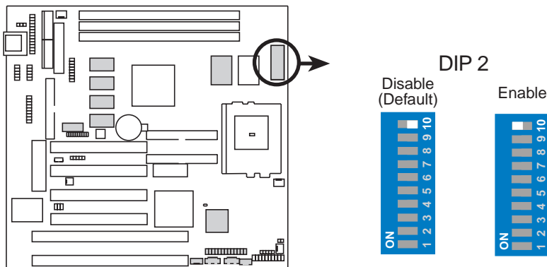
P5S-B LCD Setting
