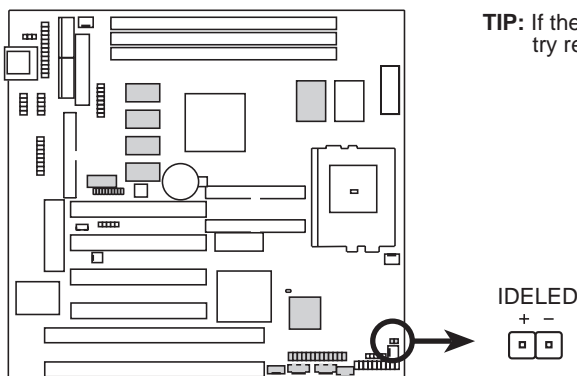
P5S-B IDE Activity LED
