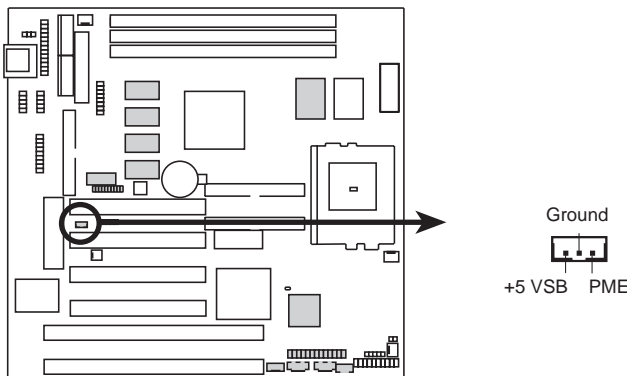
P5S-B Wake-On-LAN Connector
