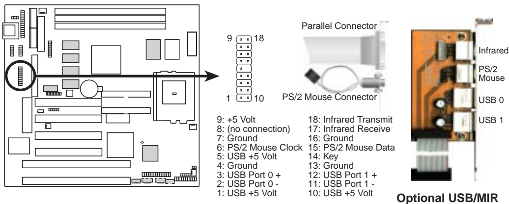
P5S-B PS/2 Mouse, USB, IrDA Module Connector
