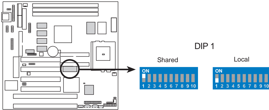
P5S-B VGA Frame Buffer Setting
