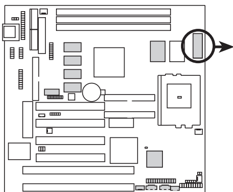
P5S-B CPU Bus Frequency Setting
