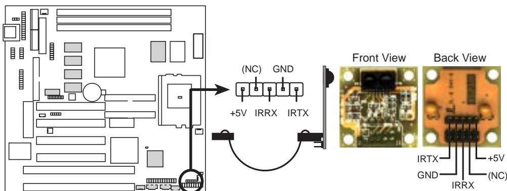
P5S-B Infrared Module Connector
