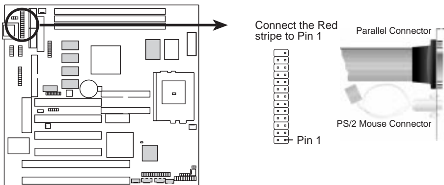
P5S-B Parallel Connector
