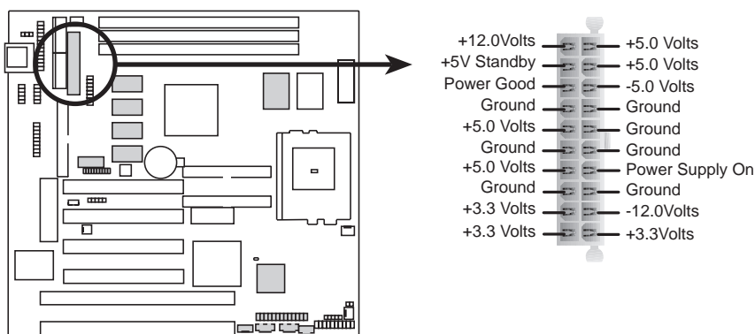
P5S-B ATX Power Connector
