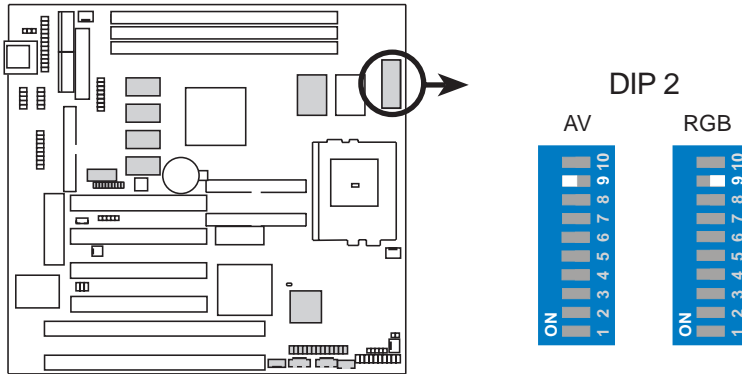
P5S-B TV Out (SCART) Setting
