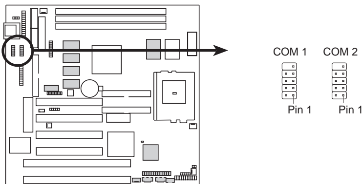
P5S-B Serial Port Connectors
