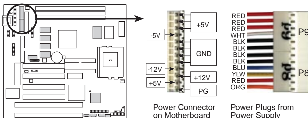
P5S-B AT Power Connector
