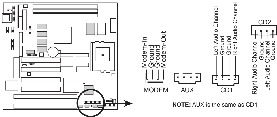
P5S-B Internal Audio Connectors
