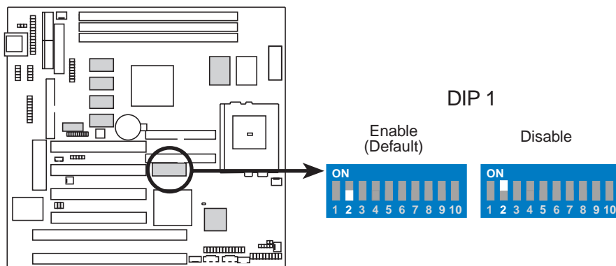
P5S-B Onboard VGA Setting
