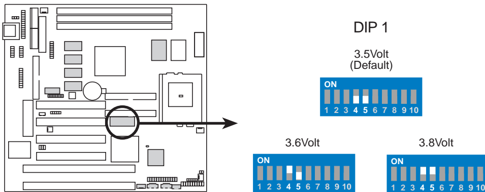
P5S-B Voltage I/O Setting
