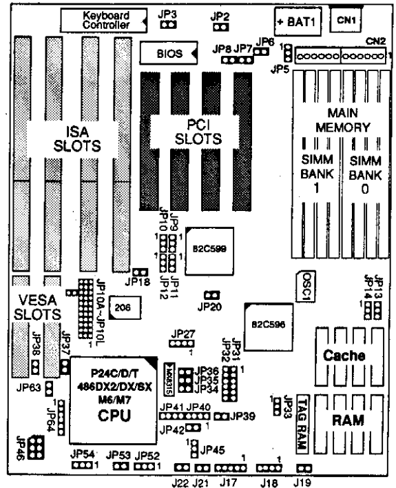
Figure 1-1. Mainboard Layout
