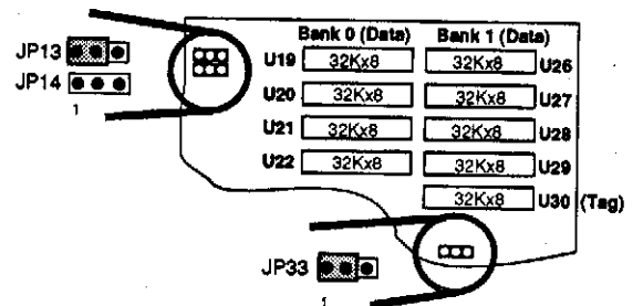
Figure 2-12. 256K Cache Configuration with 32Kx8
