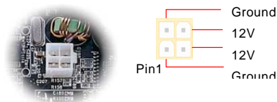
4-Pin 12V ATX Power Connector
