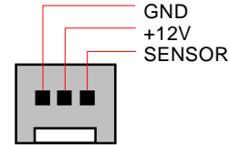
FAN2 Connector
