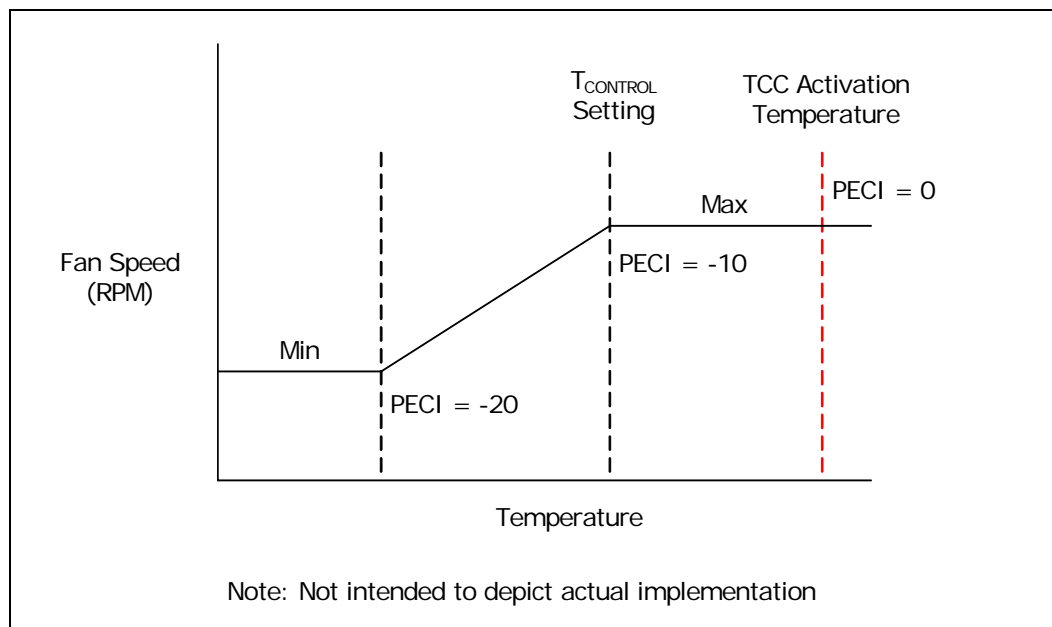
Figure 16. Conceptual Fan Control on PEFI-Based Platforms
