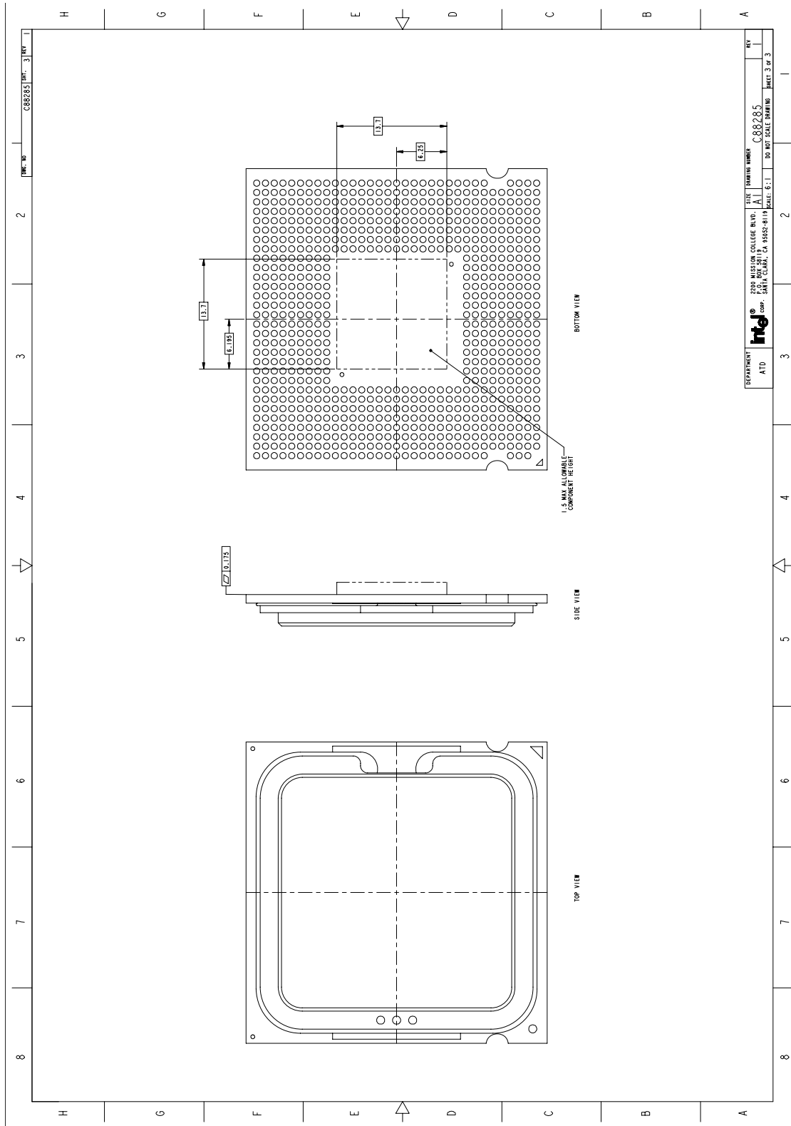
Figure 8. Processor Package Drawing Sheet 3 of 3
