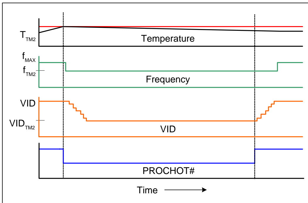
Figure 15. Thermal Monitor 2 Frequency and Voltage Ordering
