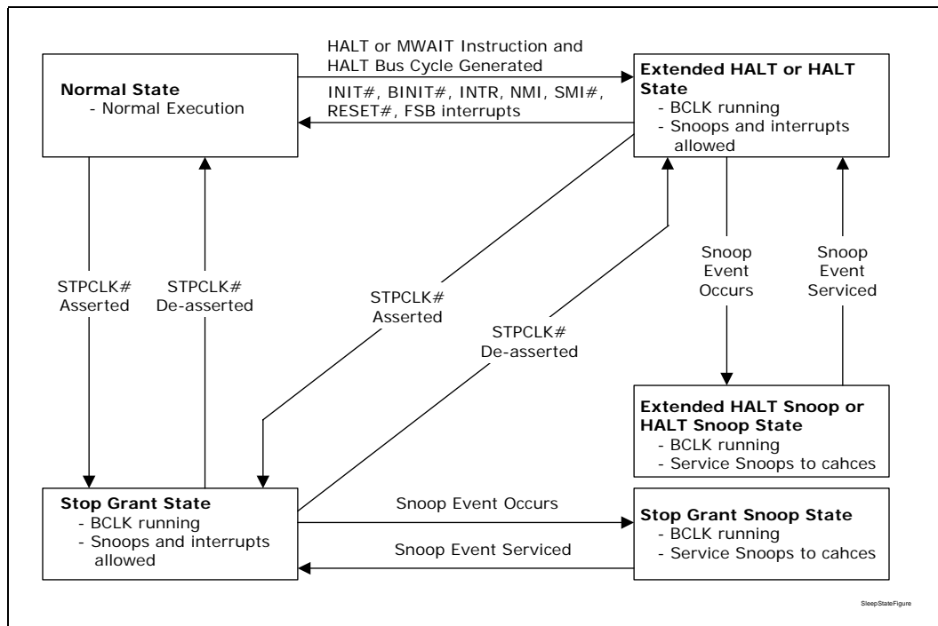
Figure 17. Processor Low Power State Machine
