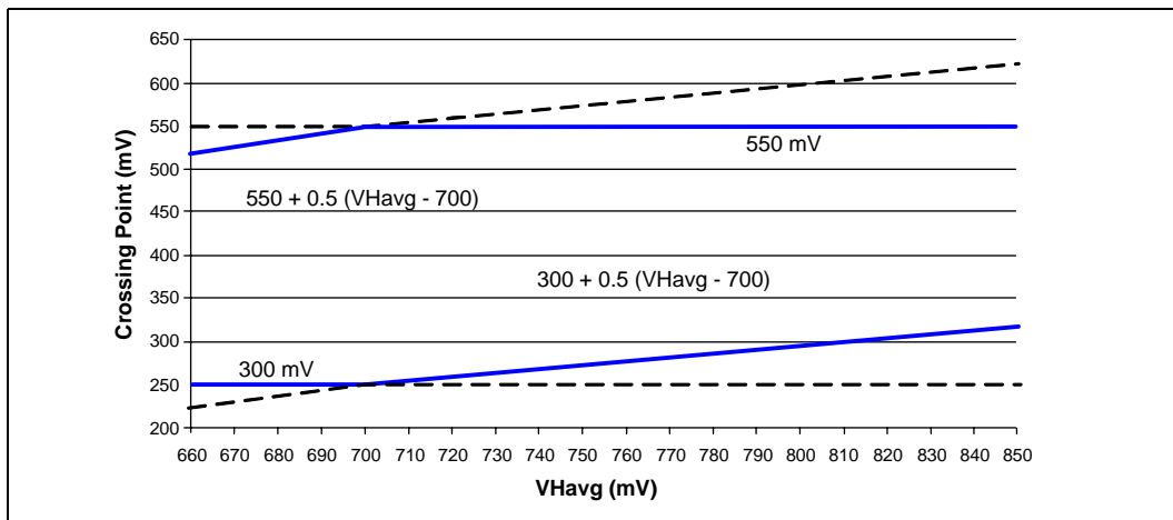
Figure 4. Differential Clock Crosspoint Specification
