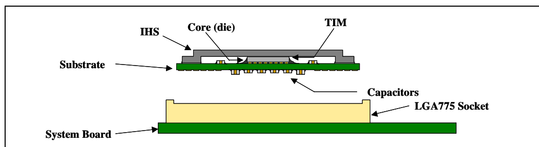
Figure 5. Processor Package Assembly Sketch
