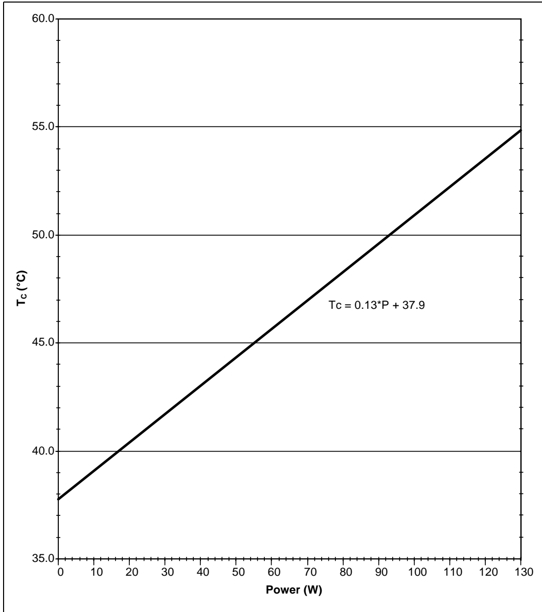
Figure 13. Thermal Profile 130 W Processors
