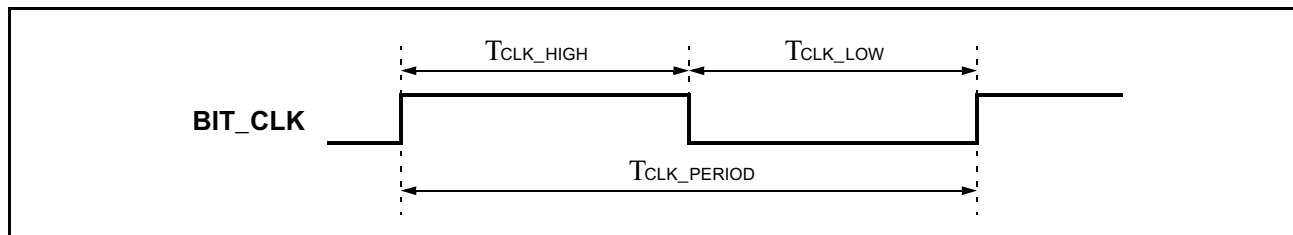
Figure 9. BIT_CLK Timing
