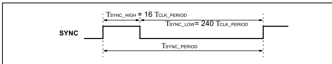
Figure 10. SYNC Timing
