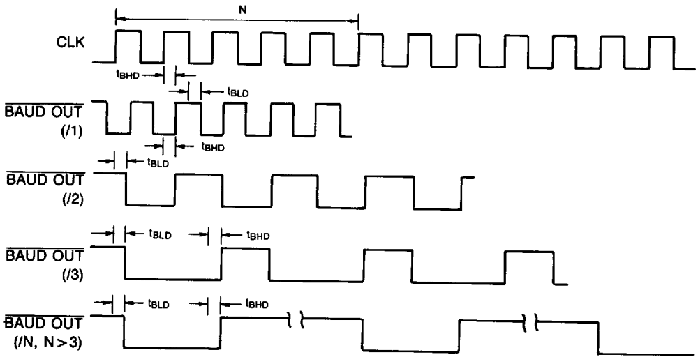
Baudout Timing
