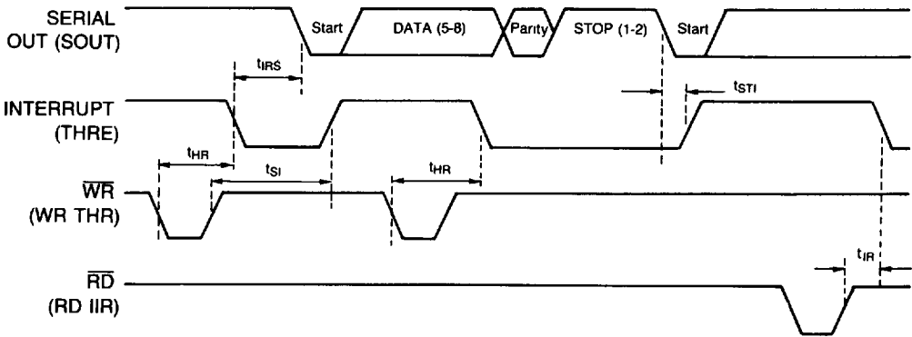
Transmitter Timing
